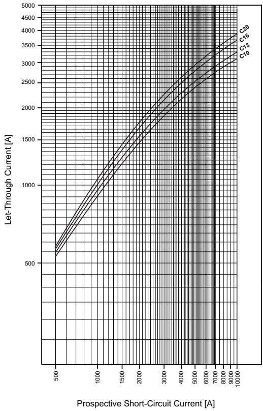
Characteristic C
