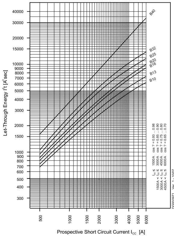
Let-through energy FRBm6, characteristic B, 2-pole
