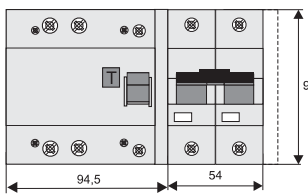
FBHmV/2p + AZ/2p
