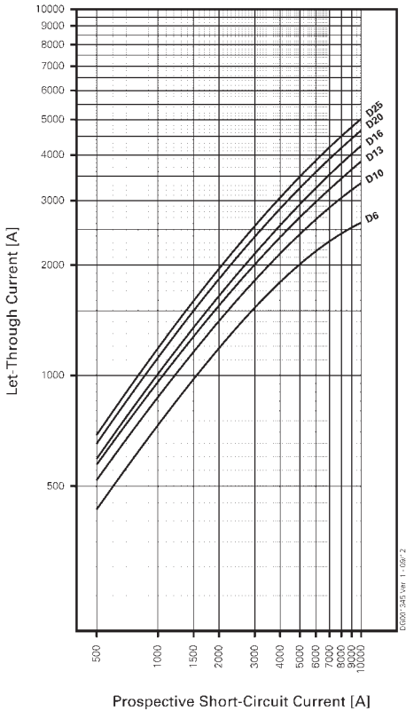
Let-through current FRBdM, characteristic D
