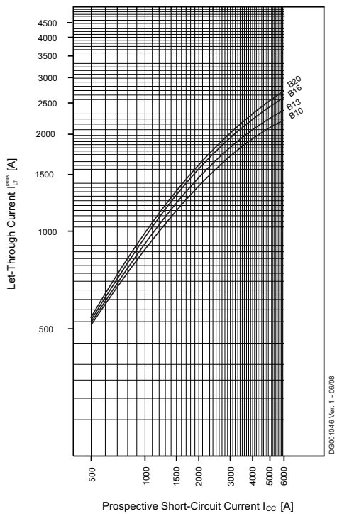
Characteristic B
