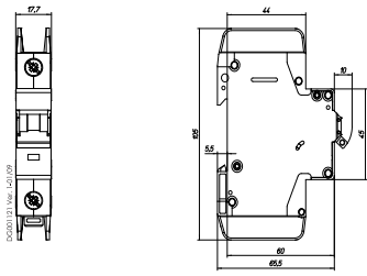
1-pole
