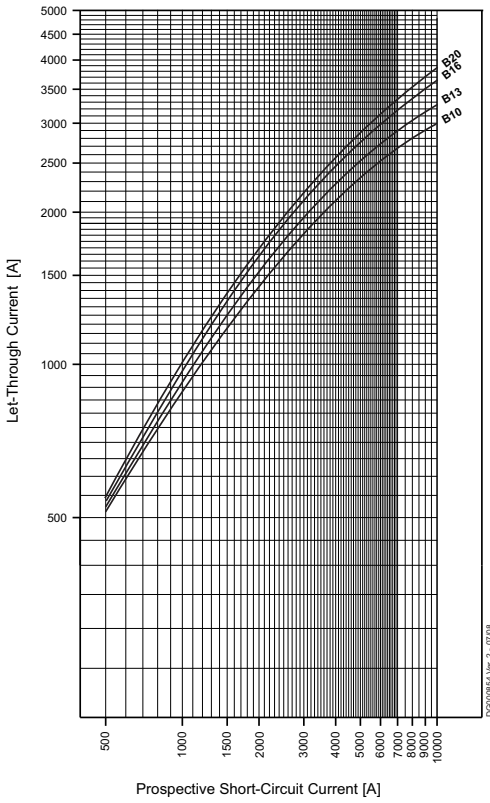
Characteristic B
