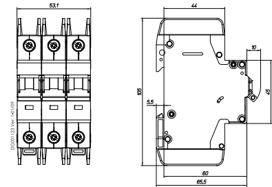
3-pole
