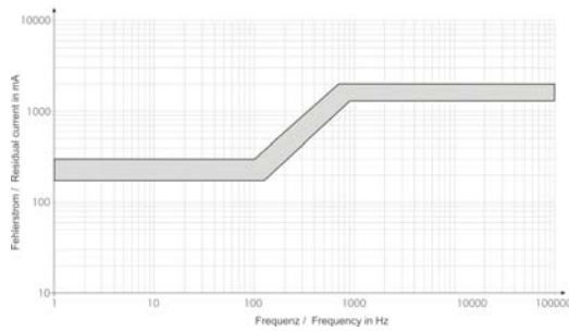
Tripping current frequency response 300 mA Type S/Bfq
