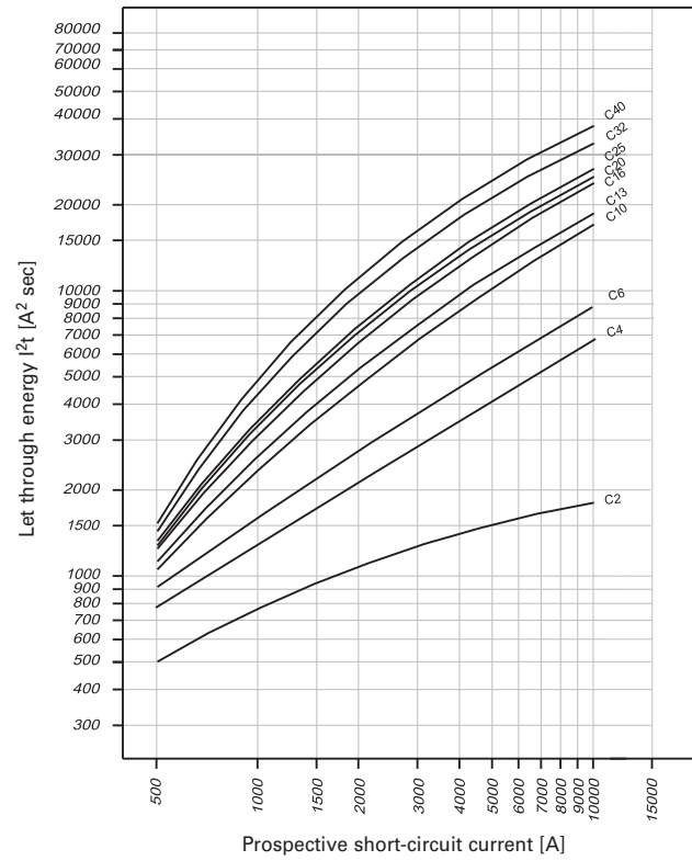
Let-through energy FRBmM, characteristic C, 1+N-pole
