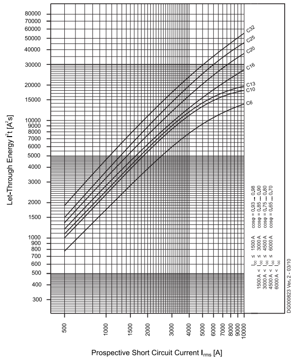
Type C
