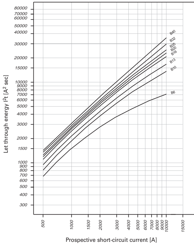
Let-through energy FRBmM, characteristic B, 1+N-pole
