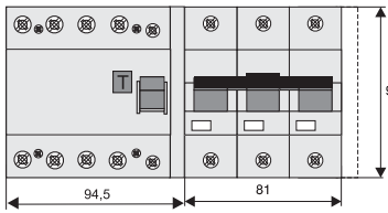
FBHmV/4p + AZ/3p
