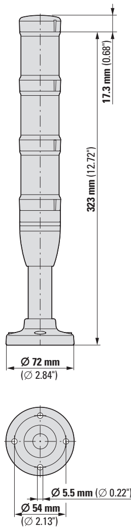
SL4-100-L-RYG-24LED
