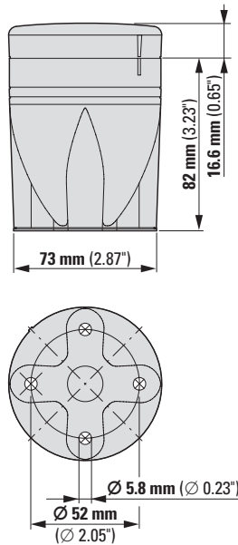
SL7-CB-IMH
